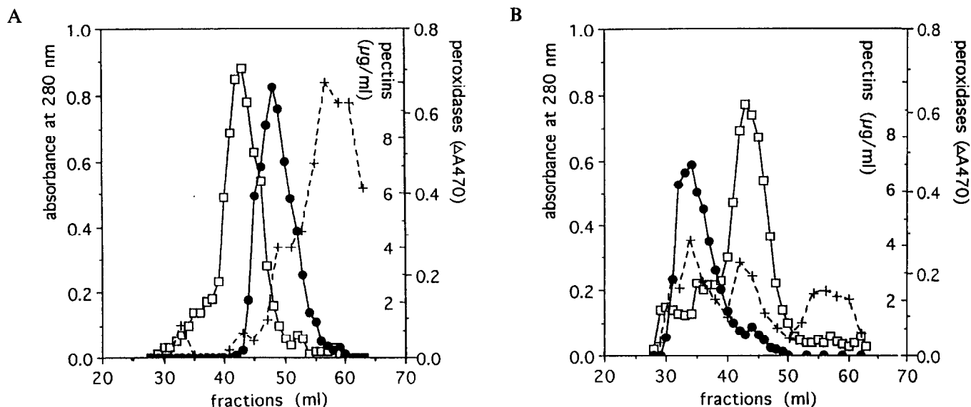
Fig. 5. Gel filtration chromatography of a crude preparation of pelletable peroxidases on Sephacryl S200. A_{280} ( \square ), peroxidase activity ( \bullet ) and pectin content (+) were determined in each fraction. (A) In presence of EGTA (10 mM in the preparation and 1 mM in the column); (B) As (A) plus \text{CaCl}_2 (7 mM in the preparation and 0.7 mM in the column).
